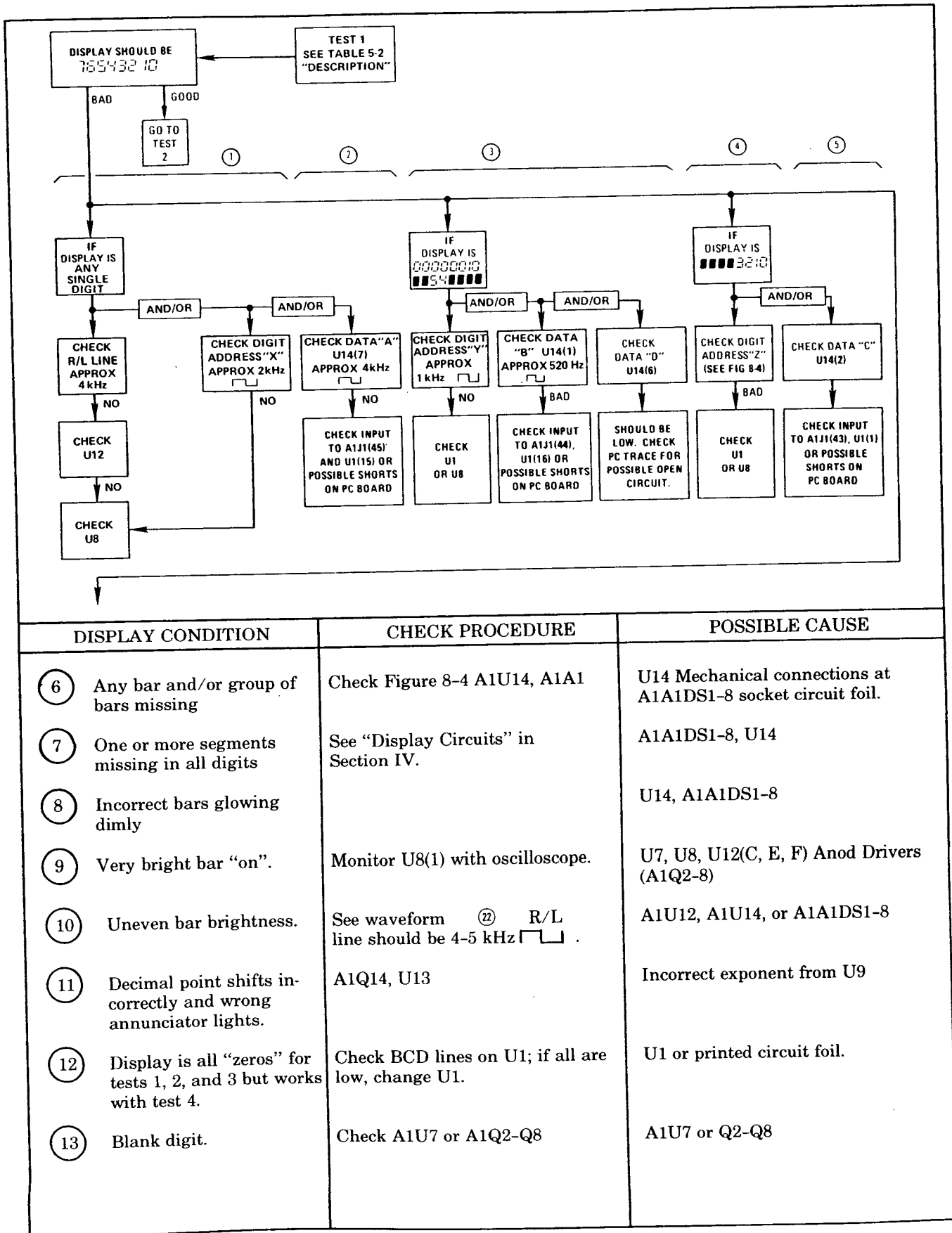
Figure 5-2. Display Checks
