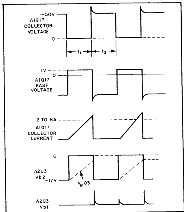
Figure 4-6. Power Supply Waveforms
